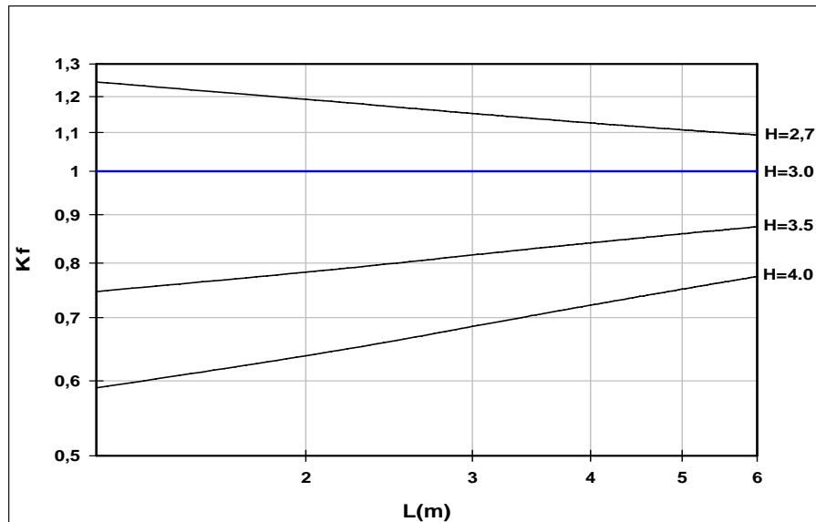
Correction factor for H ceiling different to 3 m
