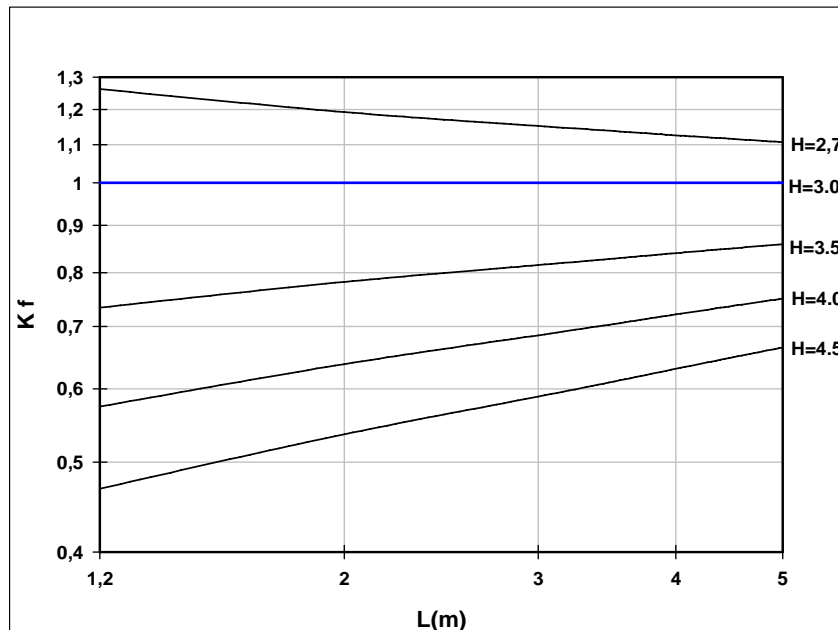
Correction factor for H ceiling different to 3 m
